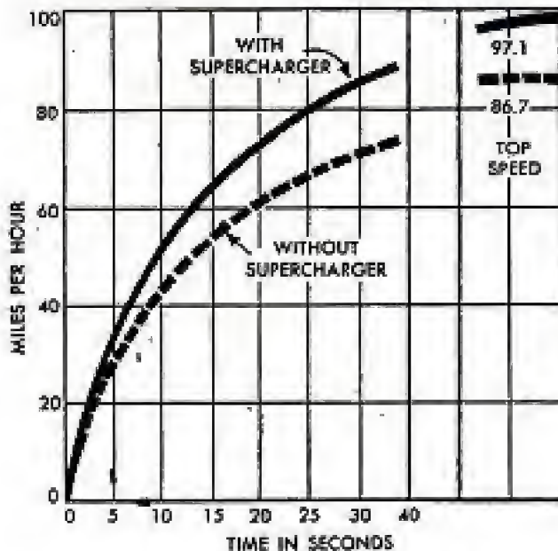
Curves mark acceleration and top speed of Mercury test car before and after supercharger was added
